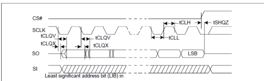
Figure 58. Output Timing
