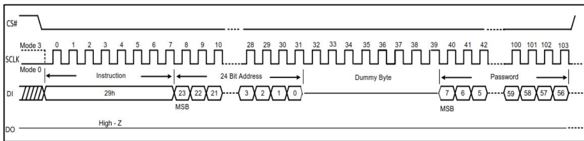
Figure 47a Unlock Password Sequence Diagram (SPI)
