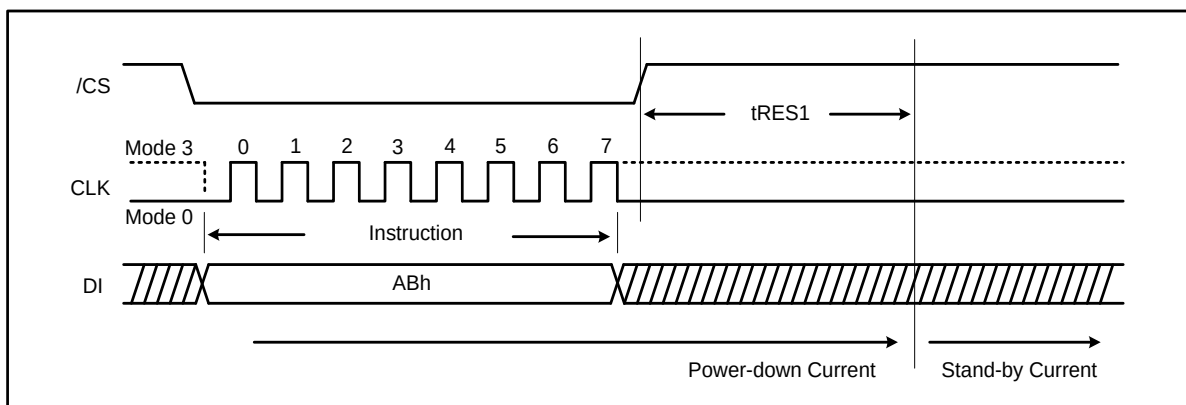
Figure 34a. Release Power-down Instruction (SPI Mode)
