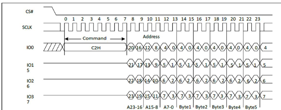
Figure 26 Extend Quad Page Program Sequence Diagram (SPI)
